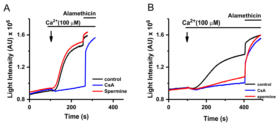
Fig. 4. Spermine does not inhibit swelling in KCl-based media, but does in the presence of NMDG ^{+} . A. Spermine does not inhibit swelling in the buffer containing 150 mM of KCl. B. When sucrose was replaced partially by an ion larger in size and unable to cross intact mitochondrial inner membranes (NMDG ^{+} ), spermine inhibited swelling. n = 3 ; experiments done in triplicate.
